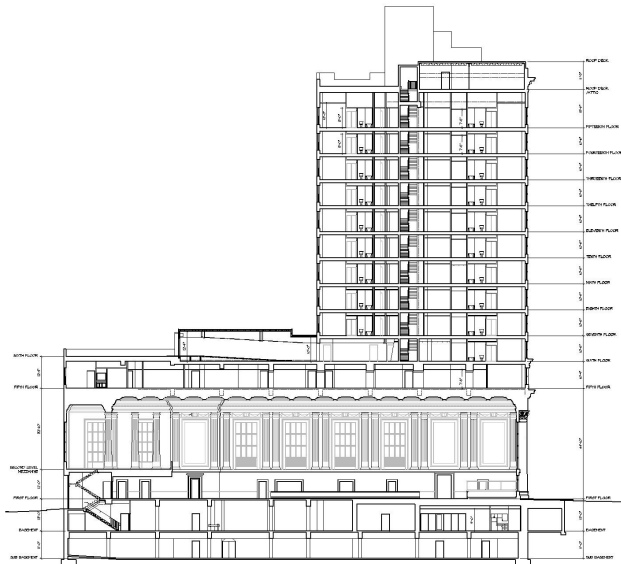
Building Section
